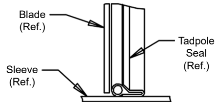
Ept. Fiberglass or Inconel tadpole seal in steel U-clip frame.
